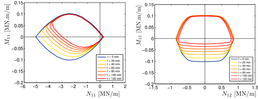
Fig. 9 Evolution of interaction diagrams at different times : left : (N_{11}, M_{11}) -plane, other N_{ij} = M_{ij} = 0 ; right : (N_{12}, M_{11}) -plane for N_{11} = -2.4 \text{ MN/m} , other N_{ij} = M_{ij} = 0
