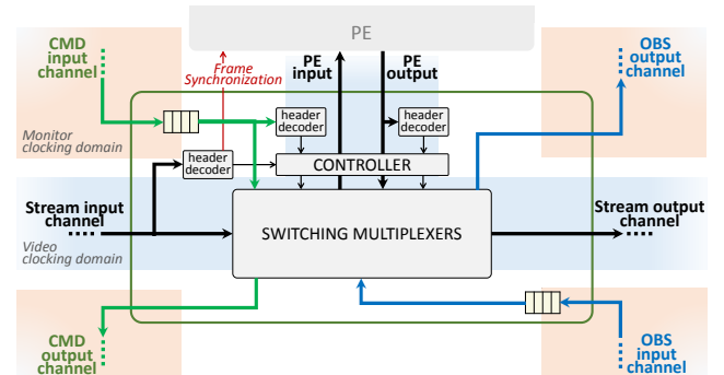
Figure 8: R_M router internal structure
