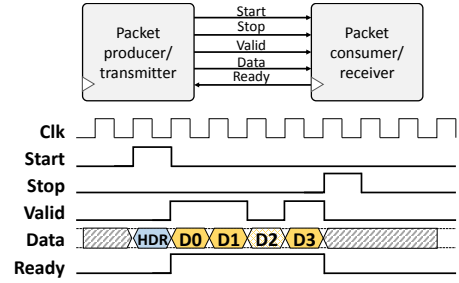
Figure 6: Communication interface and protocol
