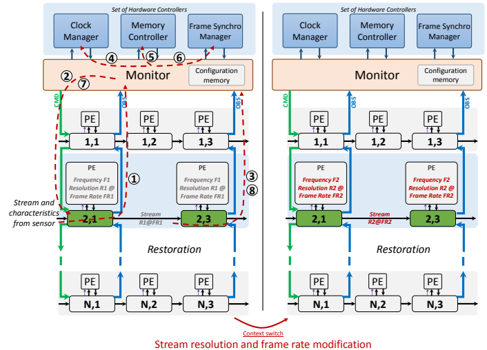
Figure 11: Stream frame rate and resolution adaptation principle
