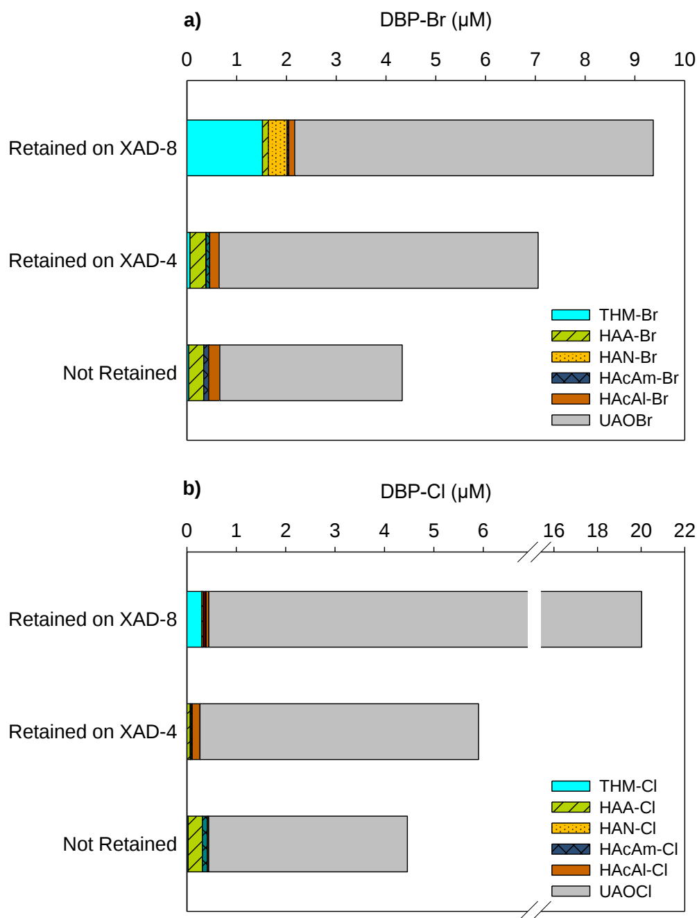
Fig. 5. DBP contributions to a) AOBBr and b) AOCl retained on XAD-8 and XAD-4 resins, based on concentrations analyzed in water samples at the inlet and outlet of each resin. UAOCi and UAObBr stand for unknown AOCl and unknown AOBBr.
