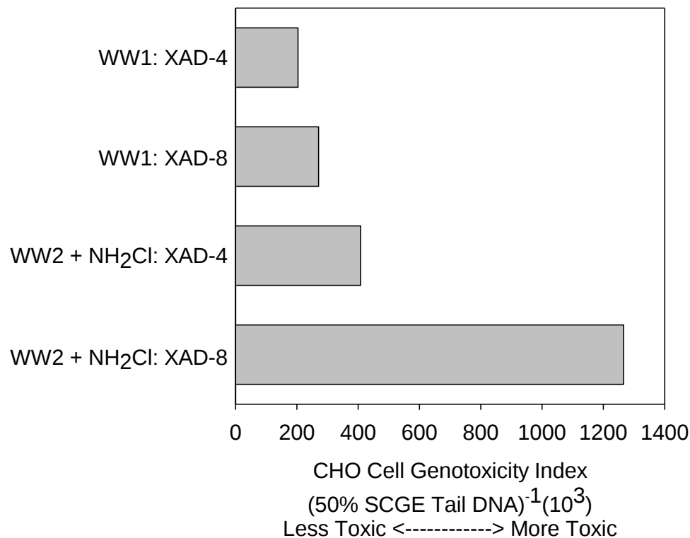
Fig. 3. Comparison of the CHO cell genotoxicity index values for each fraction of non-chloraminated wastewater effluent (WW1) and chloraminated wastewater effluent (WW2). CHO: Chinese hamster ovary. The genotoxicity data indicate that the wastewater EfOM isolated from the XAD-8 resin was more genotoxic than the XAD-4 extracts of the same wastewaters. This suggests that hydrophobic EfOM comprised more potent inducers of genomic DNA damage than transphilic EfOM. Chloramination had a major effect on the resulting genotoxicity of the XAD-8 extracted organic material, significantly more that for the XAD-4 isolate. These data indicate that the chloraminated EfOM extracted over XAD-8 or XAD-4 resins were more genotoxic than non-chloraminated EfOM.
