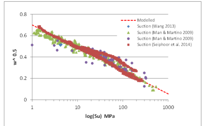
Figure 2. Linearized mass-ratio-based water retention curves for MX-80 bentonite from various sources
