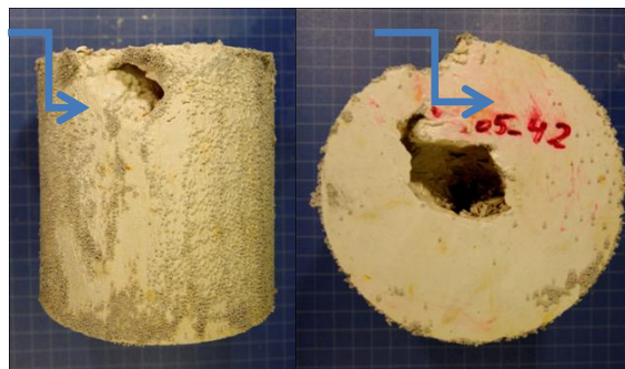
Figure 1. Typical liquefaction type failure on hollow cylinder on brine saturated Mons chalk. Arrows indicate the location of the failure area.
