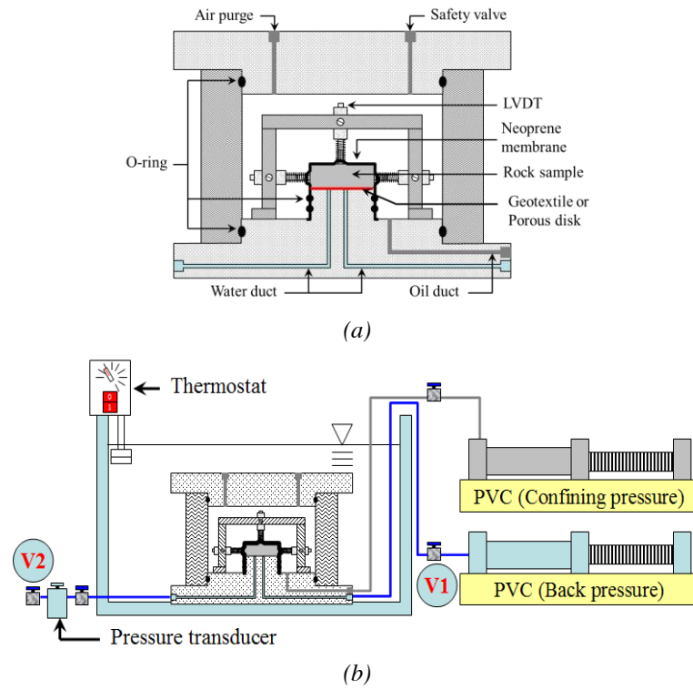
Figure 1. (a) Isotropic compression cell; (b) Overall system with controlled temperature bath
