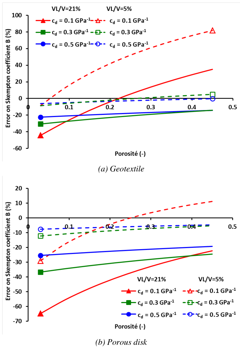
Figure 10. Parametric study of the error on Skempton coefficient (B)
