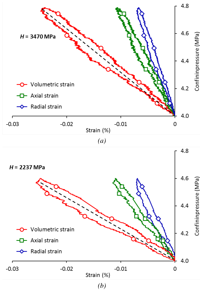
Figure 9. Pore pressure loading-unloading test: (a) EST31912c, (b) EST31912e.
