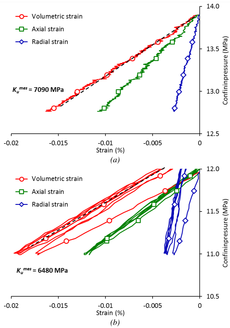
Figure 7. Undrained isotropic compression tests: (a) EST31912c, (b) EST31912e.
