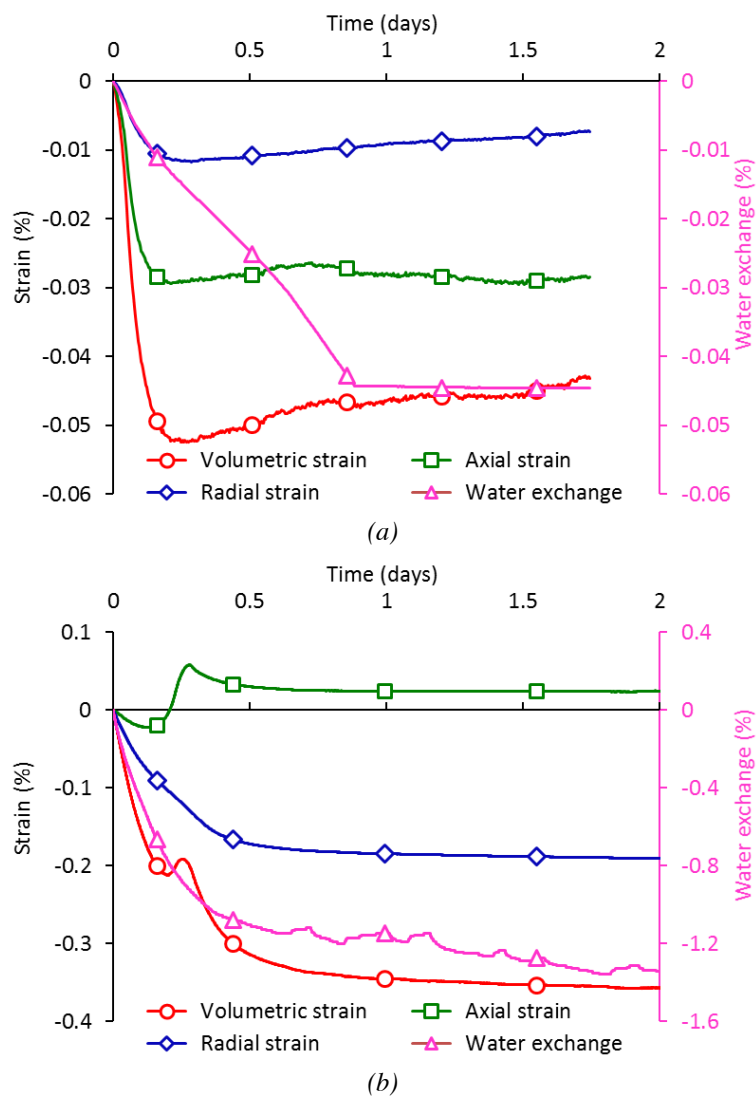
Figure 4. Saturation phase: (a) sample EST31912c, (b) sample EST31912e.
