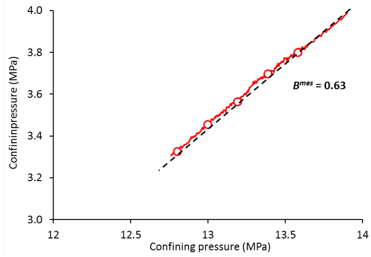
Figure 6. Skempton coefficient measured for test EST31912c
