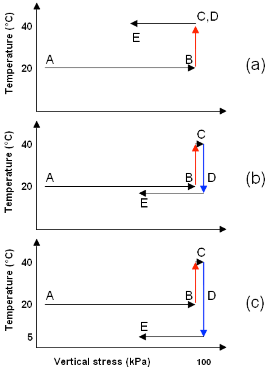
472 Figure 5. Thermo-mechanical paths: (a) tests at 40°C; (b) tests at 20°C; (c) tests at 5°C
