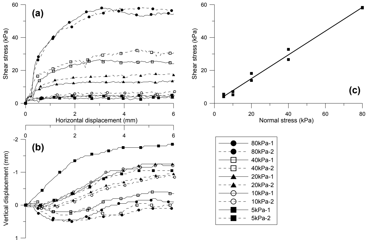
479 Figure 6. Experimental results on sand at 5°C: (a) Shear stress versus horizontal 480 displacement; (b) Vertical displacement versus horizontal displacement; (c) Shear strength 481 envelope
