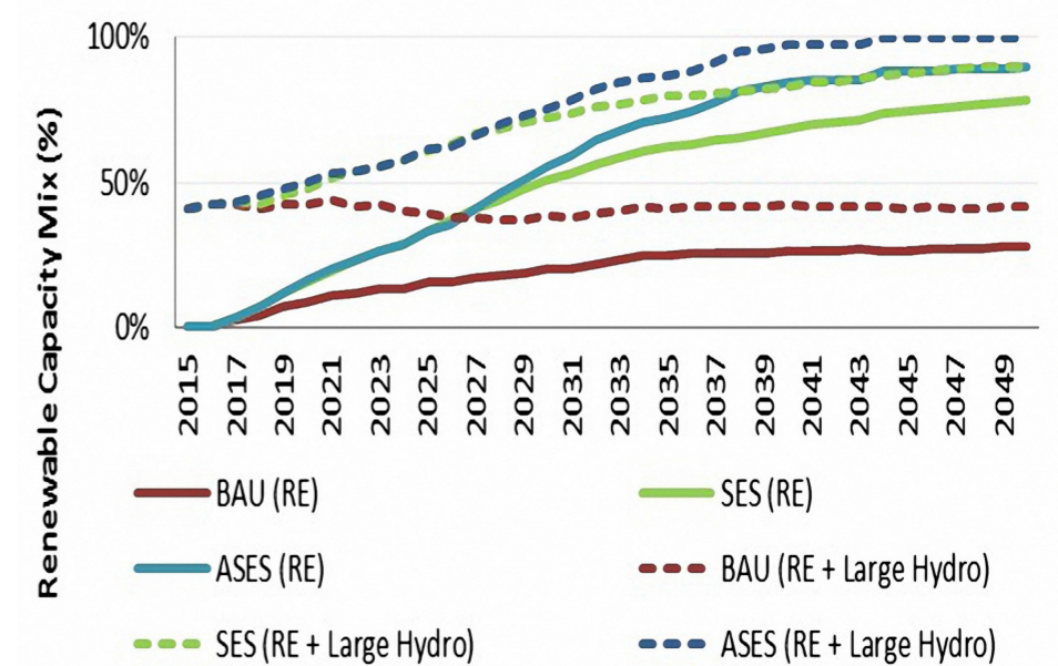
Figure 14: Viet Nam Renewable Installed Capacity Mix
