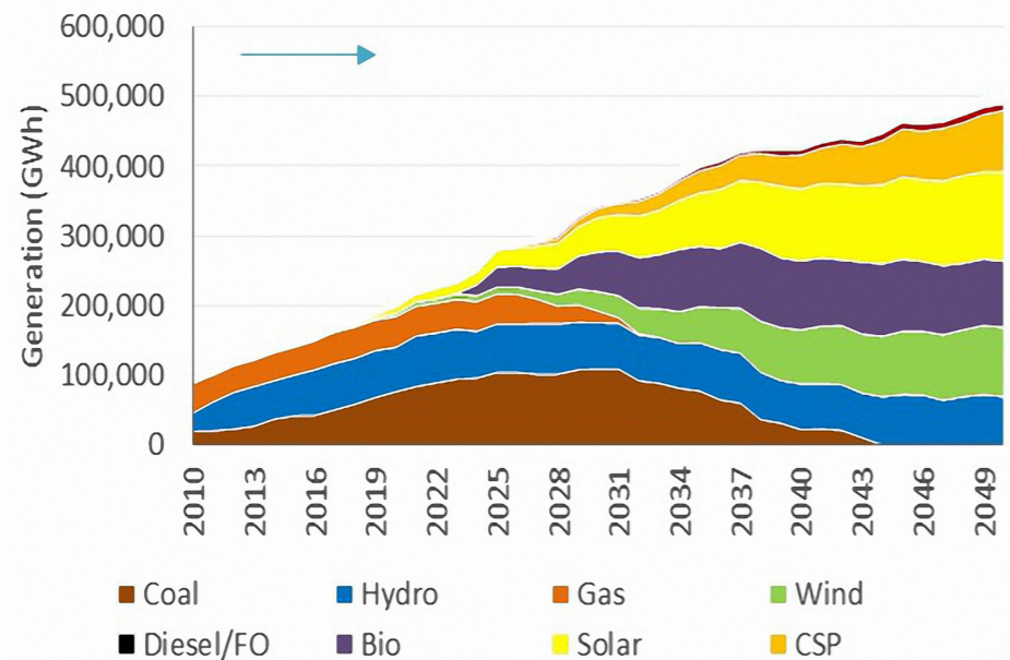
Figure 13: Viet Nam Generation Mix (ASES, GWh)
