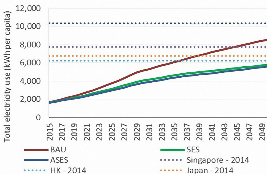
Figure 8: VietNam Per Capita Consumption Comparison (kWhpa)
