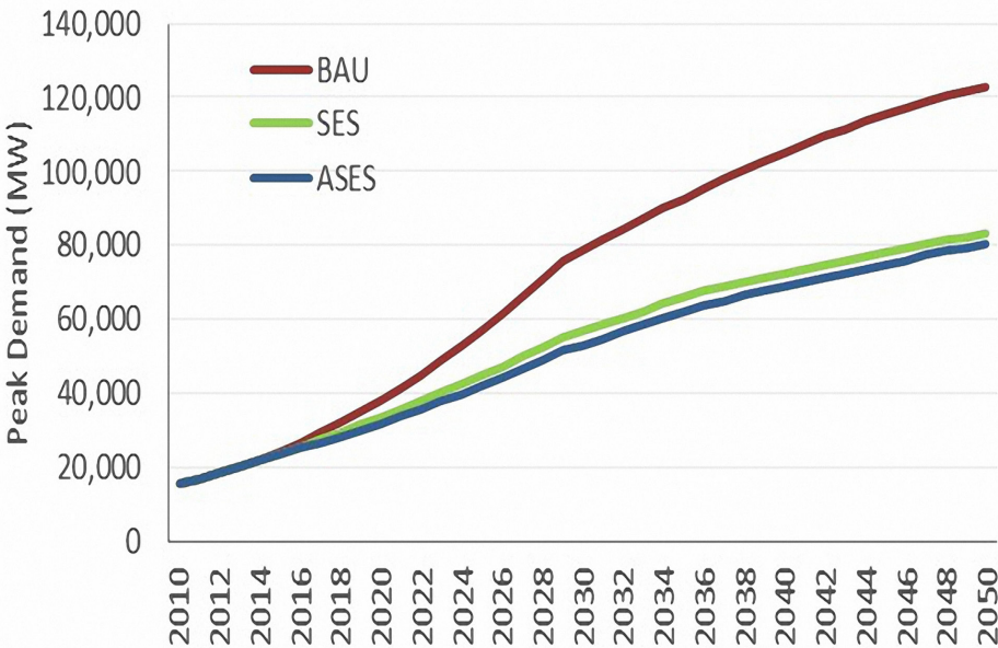
Figure 7: Viet Nam Peak Demand Comparison
