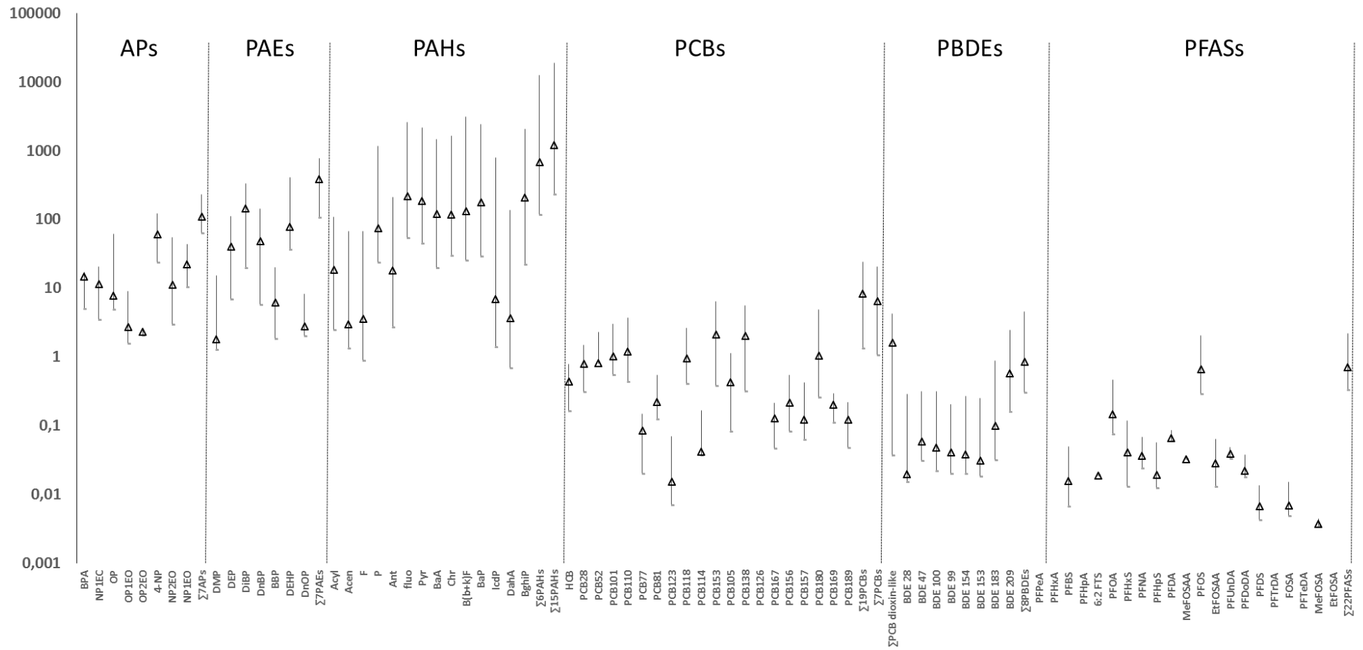
Figure 3: Organic micropollutant contents in soils (d10, d50 and d90, as µg/kg.dw, n=31-32)
