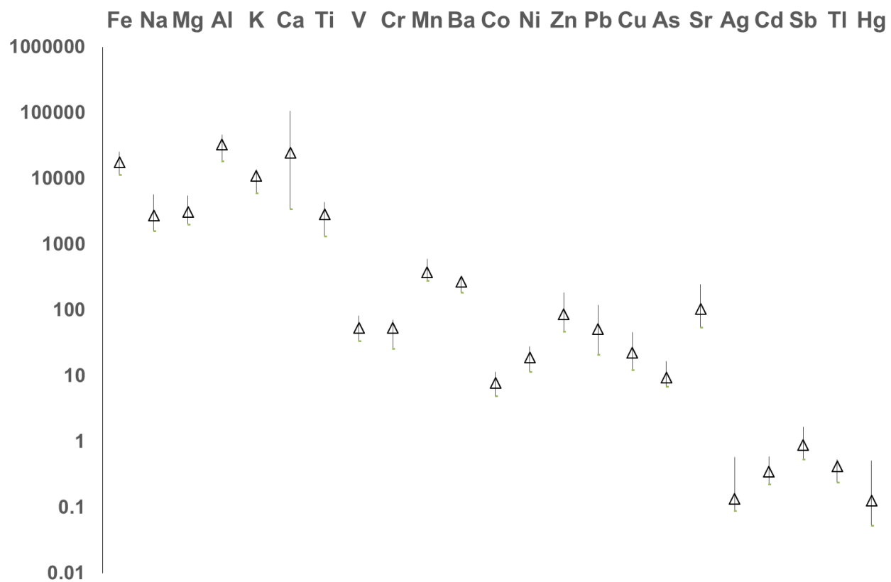
Figure 2: Metal contents in soils (d10, d50 and d90, as mg/kg.dw, n=32)
