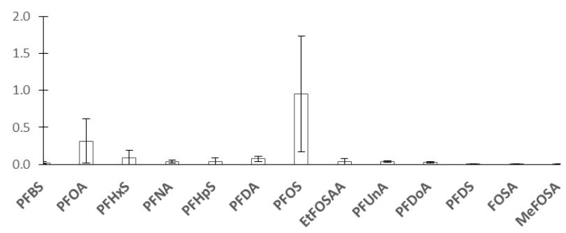
Figure 4: Organic micropollutant patterns in soils (mean \pm SD, as \mu\text{g/kg.dw} , n=31-32)
