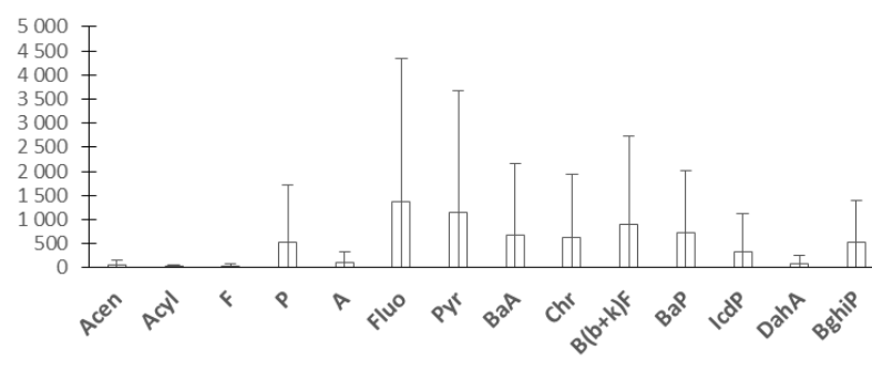
Figure 4: Organic micropollutant patterns in soils (mean ± SD, as µg/kg.dw, n=31-32)
