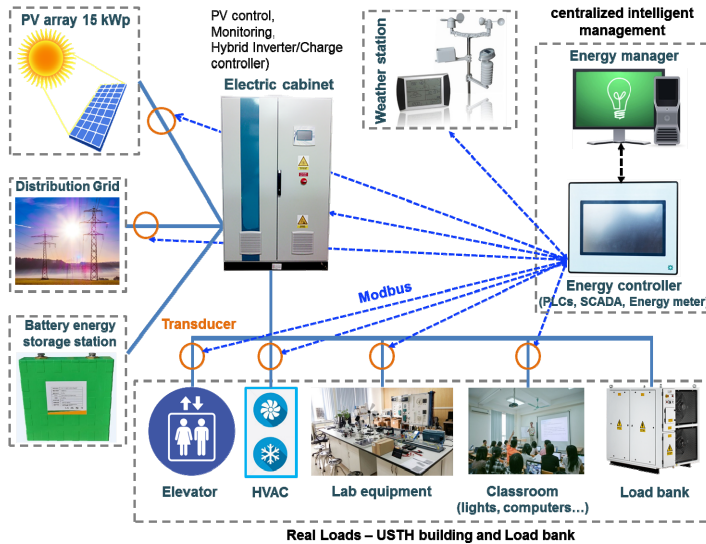
Fig. 1. Building energy management platform for University building
