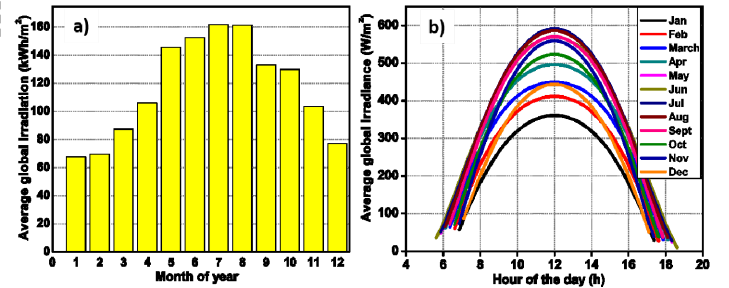
Fig. 2. Value of average global irradiation in kWh/m 2 from Meteonorm (a) and in W/m 2 from Climate-SAF PVGIS (b)
