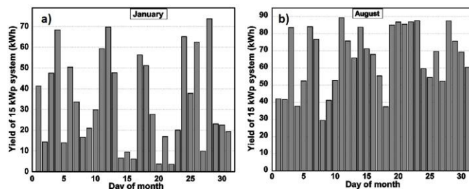
Fig. 8. Average daily yield of 15 kWp PV array for January and August.
