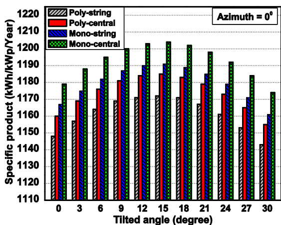
Fig. 4. Specific product of PV system for A_m = 0^0 by tilted angles
