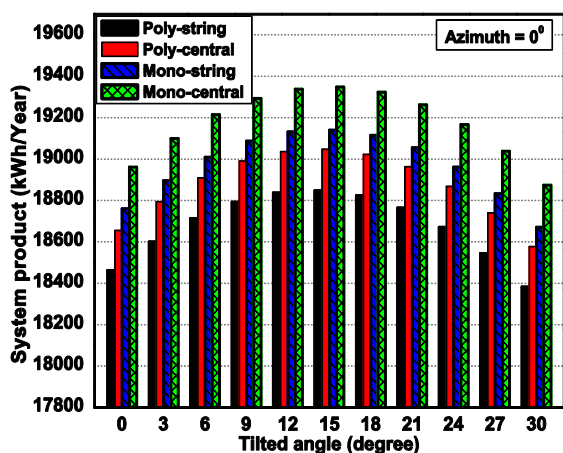
Fig. 5. System product of PV system for A_m = 0^0 by tilted angles
