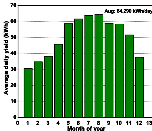
Fig. 7. Average daily yield of 15 kWp PV array for different months.
