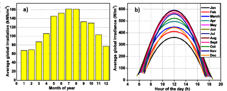
Fig. 2. Value of average global irradiation in kWh/m 2 from Meteororm (a) and in W/m 2 from Climate-SAF PVGIS (b)
