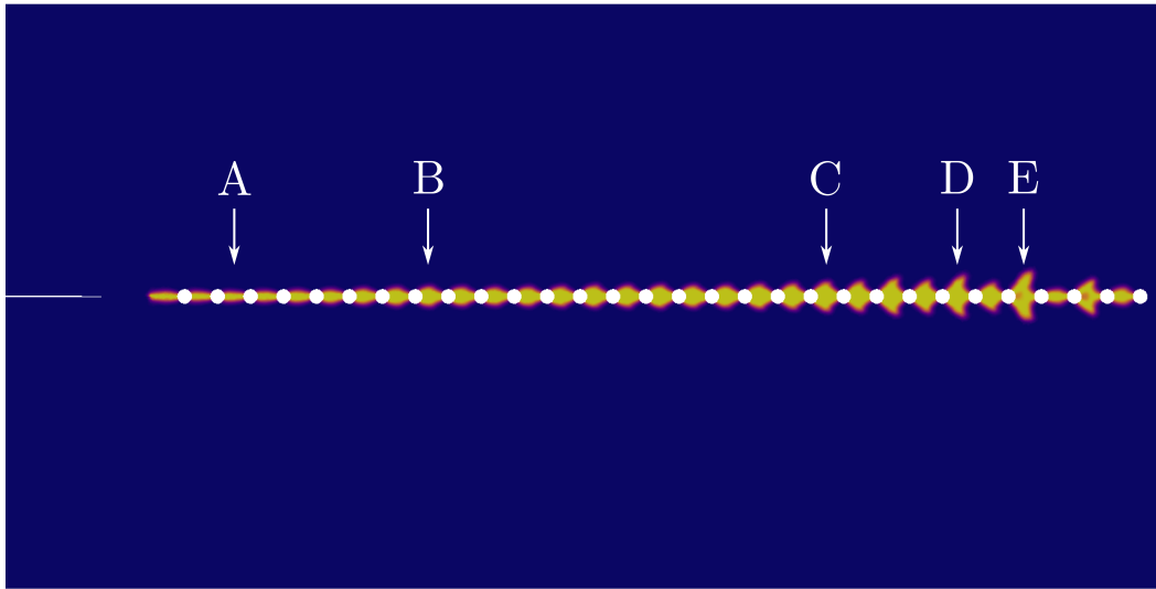
Fig. 14 Crack propagation in a perforated material with \Delta U = 0.05 mm (the same colormap as in Fig. 5 is used). Macro-branching is temporarily suppressed by crack tip attraction to the holes. Small attempts of branching can be observed at the end (events D and E). See also Movie 1 in supplementary material.
