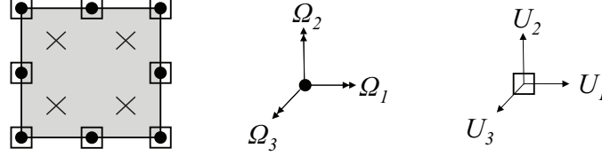
Figure 5. The quadratic micropolar plate element COSS8R [14].
