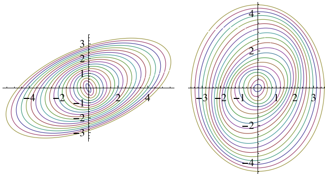
FIG. 6. Contours of 2D balls B_\lambda for scale ratios \lambda \in (1/4, 5) by steps of \delta(1/\lambda) = 0.2 and a pseudo-quaternion generator: (a, on the left) for a dominant stratification ( Q(G) > 0 ), nevertheless with some rotation ( d = 1, c = f = 0.2, e = 0.1 ); (b, on the right) for a dominant rotation ( Q(G) < 0 ), although with some stratification ( d = 1, c = f = 0.2, e = 0.7 ).
