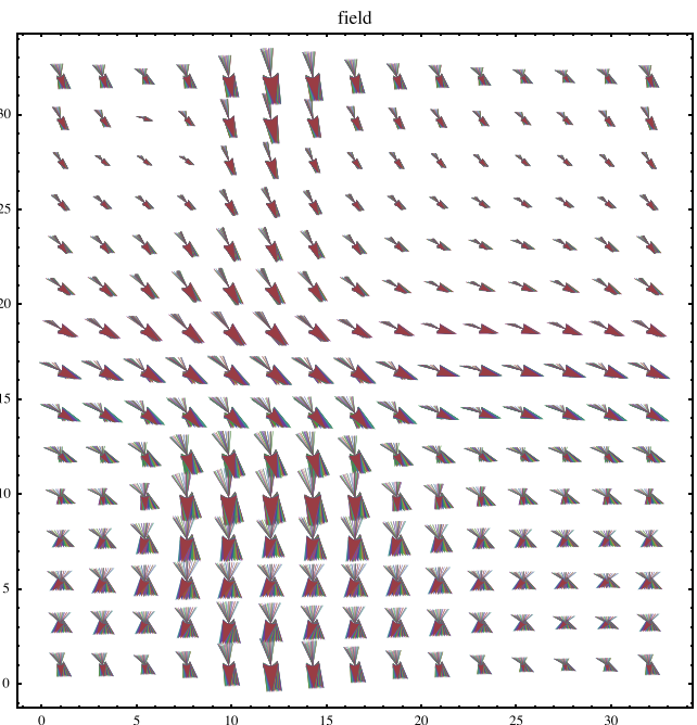
FIG. 8. Snapshot of a multifractal simulation of a 2D + 1 intermittent vector field obtained by a complex cascade, i.e., with values on Cl(0, 1) , see text for the details of the numerical simulation.
