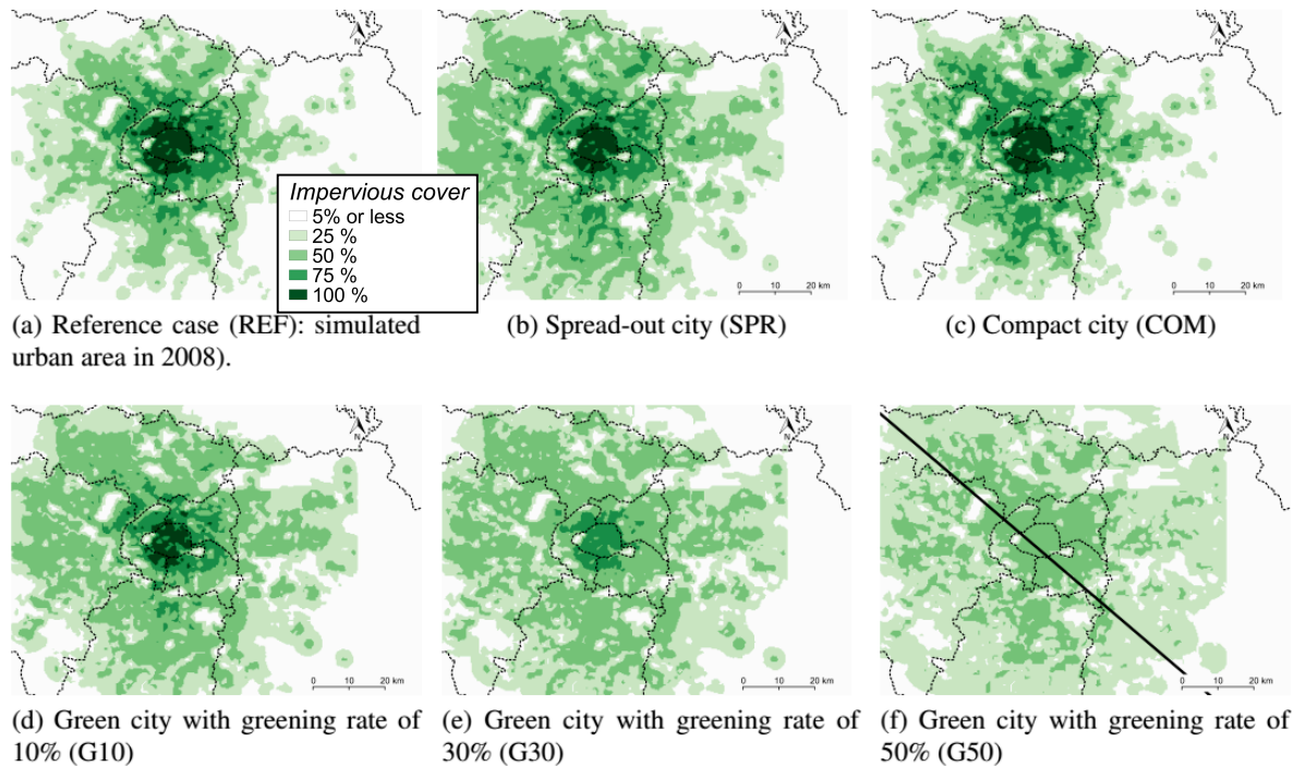
Fig. 3. Presentation of the REF case (in 2008) and the five urban sprawl scenarios, in 2100. The maps present the simulated fraction of impervious covers over the study area. The thick black line in the last map shows the line along which the profile graphs are computed in Fig. 4.
