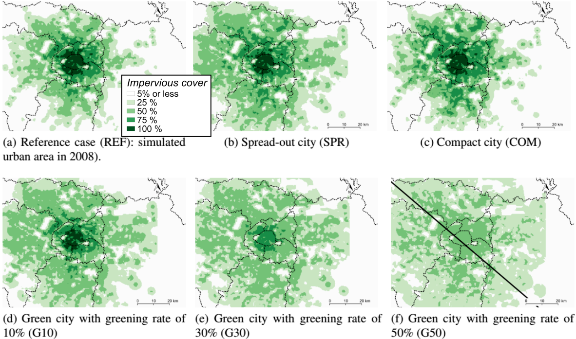
Fig. 3. Presentation of the REF case (in 2008) and the five urban sprawl scenarios, in 2100. The maps present the simulated fraction of impervious covers over the study area. The thick black line in the last map shows the line along which the profile graphs are computed in Fig. 4.
