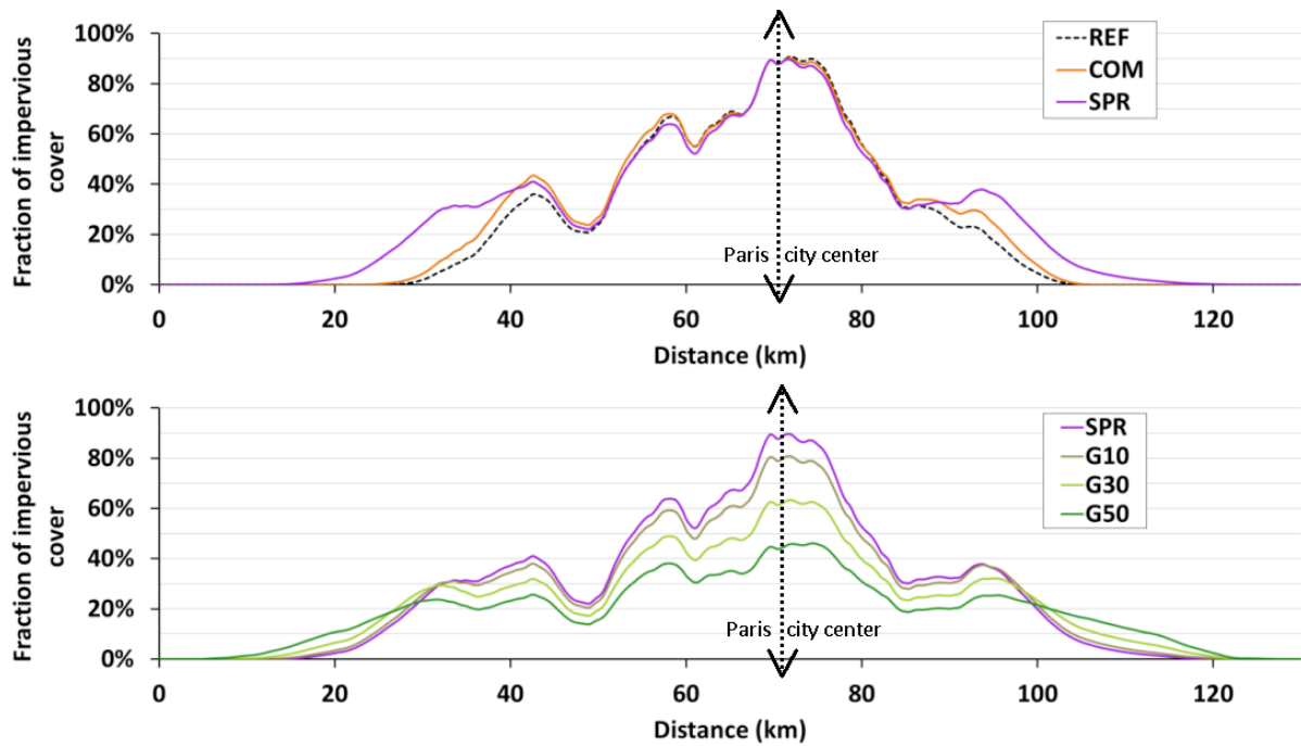
Fig. 4. Examples of impervious cover profiles over the study area.
