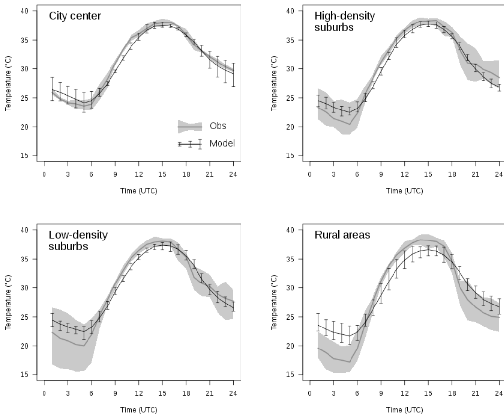
Fig. 6. Comparison between observed and modeled 2-m air temperatures on the 10 August 2003 averaged for the four land cover classes. The standard deviations are also presented both for model outputs (black bars) and observations (gray envelop).
