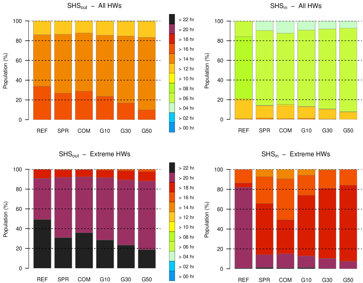
Fig. 14. Distribution of population according to the number of hours per day spent in strong heat stress for outdoor (left) and indoor (right) conditions for the different city scenarios. Results are weighted by the occurrence probabilities of all future heat waves (top) and of the most extreme ones (bottom).
