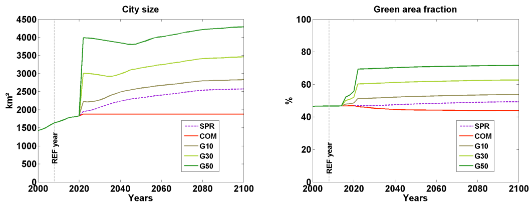
Fig. A2. City size (left) and green area fraction (right) in the scenarios.
