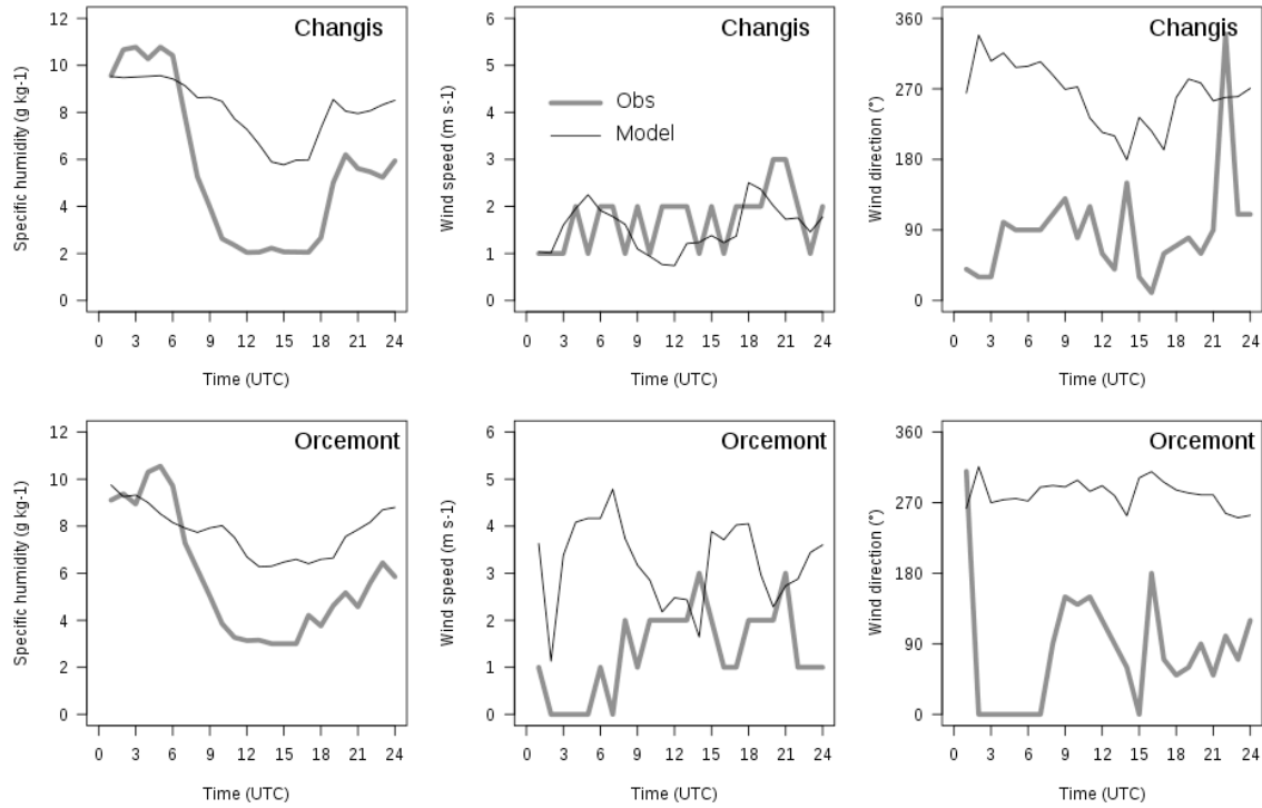
Fig. 7. Comparison between observed and modeled 2-m specific humidity, and 10-m wind speed and direction on the 10 August 2003 for the two rural stations of Changis (top) and Orcemont (bottom) located north-east and south-west of Paris, respectively.
