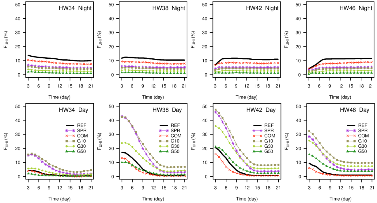
Fig. 12. Comparison of the evolution with time (from three to 21 days) of the proportion of the city affected by a UHI of 1.5°C for the today city and the future scenarios. The results are presented for the four classes of heat-wave intensity, and both for nighttime (top) and daytime (bottom) hours.
