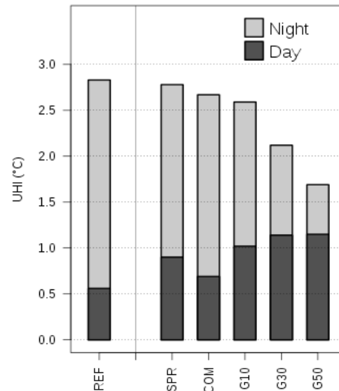
Fig. 10. Comparison of the values of UHI obtained by aggregating the results for the city-center grid points for each scenario for the HW38 after seven days of heat wave.
