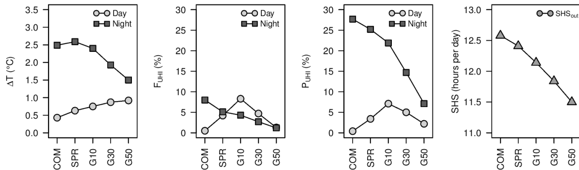
Fig 15. Example of the indicators computed for the HW38 event after 14 days for the five scenarios of urban expansion.
