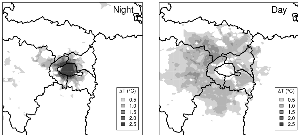
Fig. 8. Spatial representation of the city's areas affected by UHI for the different thresholds in temperature anomaly. Example of the today city ( REF scenario) for the HW38 after seven days of heat wave both for nighttime (left) and daytime (right) hours.
