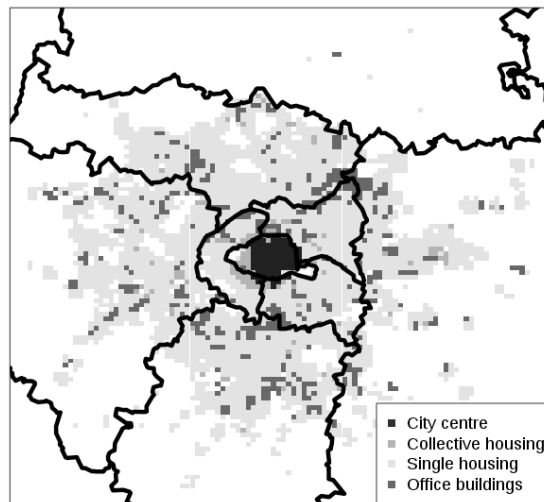
Fig. A3. Typologies of urban landscapes over the study domain, in the case of the spread-out city (SPR).
