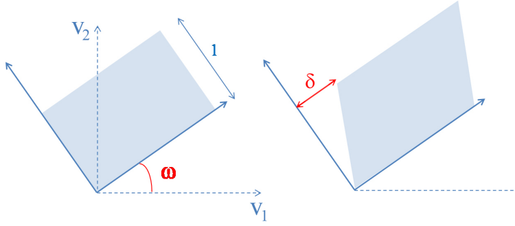
Fig. 1 Representation of the deformation \mathbf{I} + \delta \mathbf{u}(\omega) \otimes \mathbf{v}(\omega) : reference (left) and deformed (right) configuration.
