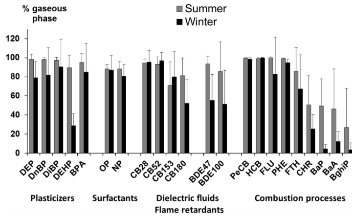
Fig. 2: Compound distribution in the gaseous phase as % of total (mean \pm SD, n = 9), at the three sites, during summer and winter.
