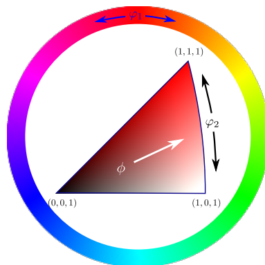
Fig. 9. Hue-Saturation-Value (HSV) colour coding for cubic crystal orientation: Hue, Saturation and Value correspond to the traditional Bunge angles \varphi_1 , \varphi_2 and \phi .
