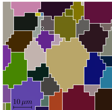
Fig. 7. Grain orientation mapping of the strain-free substrate, calculated on the main spots for a \text{UO}_2 polycrystal implanted with 60 keV Helium ions at 10^{16} ions/cm 2 . The corresponding colours follow HSV convention described in Appendix A.
