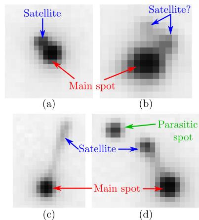
Fig. 4. Four cases of difficult satellite detection in Laue pattern measured on He-implanted \text{UO}_2 polycrystals: (a) satellite close to the main spot; (b) complicated satellite shape near the grain boundaries; (c) elongated satellite for high implantation fluence; (d) presence of a parasitic spot.
