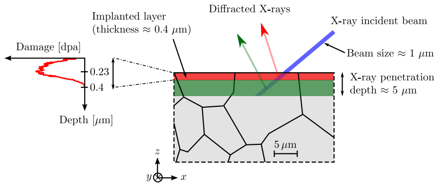
Fig. 1. Schematic representation of a polycrystalline sample implanted in a thin surface layer, marked out in red. The estimated damage profile, due to Helium implantation at 60 keV, is represented along the depth. The X-ray incident beam is diffracted by the damaged layer and the strain free substrate.
