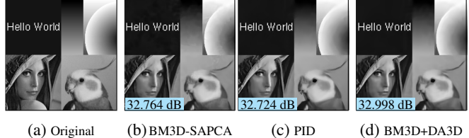
Fig. 3: Denoising results for Montage , \sigma = 25 . A zoom-in is advised to see the staircasing effects in (b) and (c) and their removal in (d).
