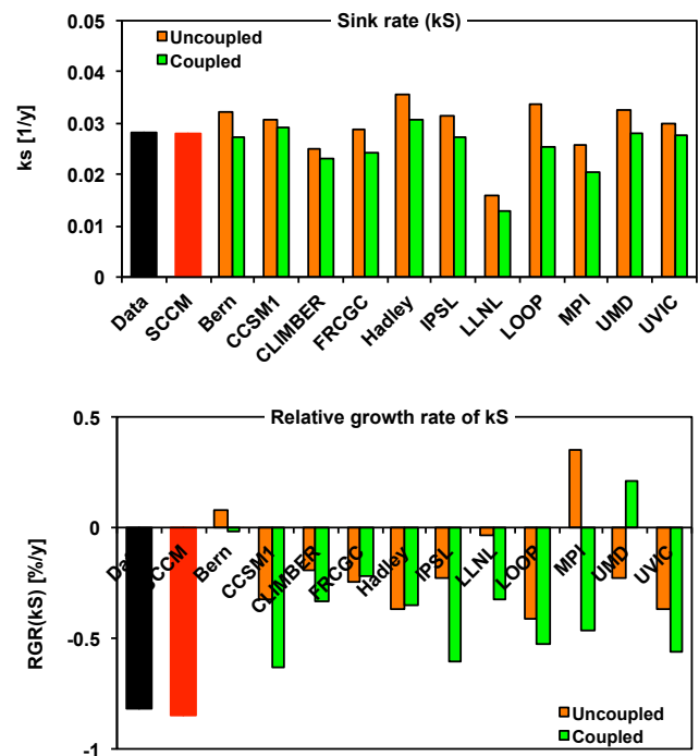
Figure 9. Upper panel: mean sink rate k_S over 1959.0–2013.0 from data (black bars), SCCM (red bars) and 11 C4MIP models (Friedlingstein et al., 2006) in both uncoupled and coupled modes (orange and green bars, respectively). Lower panel: relative growth rate RGR( k_S ), estimated using Eq. (A2). See Fig. 8 caption for note on consistency of SCCM trend estimates between Figs. 9 and 3.
