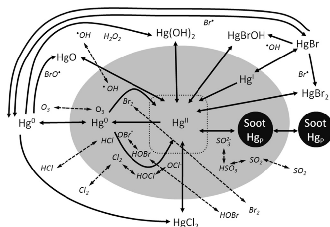
Fig. 1. The implemented chemical model for mercury. In this picture the gaseous and aqueous phases are marked by white and grey, respectively. The line arrows show possible transformations of mercury. The dashed arrows show additional species used in the model which react with mercury.
