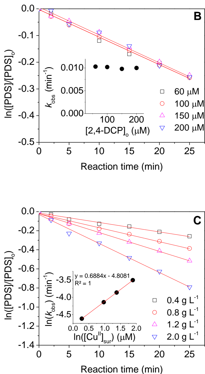
Figure 5. Influences of PDS dose on 2,4-DCP decomposition (A: [2,4\text{-DCP}]_0 = 5 \mu\text{M} , CuO dose = 400 \text{ mg L}^{-1} ), 2,4-DCP dose on PDS decomposition (B: [\text{PDS}]_0 = 20 \mu\text{M} , CuO dose = 400 \text{ mg L}^{-1} ), and CuO dose on PDS decomposition (C: [\text{PDS}]_0 = 20 \mu\text{M} , [2,4\text{-DCP}]_0 = 10 \mu\text{M} ) during PDS/CuO oxidation. Conditions: \text{pH} = 5.8 , T = 20 \text{ }^\circ\text{C} .
