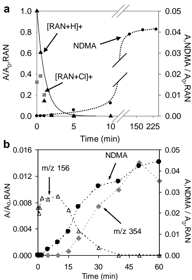
251 Figure 3. Decomposition of ranitidine (a) and formation of NDMA and other by-products (a and b) by 252 chloramination monitored by HPLC-MS in APCI positive mode. [\text{RAN}]_0 = 12 \mu\text{M} ; [\text{NH}_2\text{Cl}]_0 = 2.5 \text{ mM} ;
