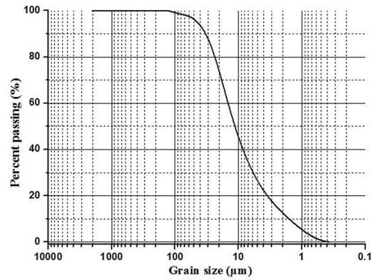
Fig. 3 Particle size distribution curve of the soft clay
