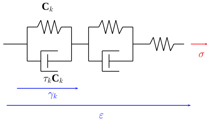
Figure 2: A rheological model made of a series of Kelvin chains
