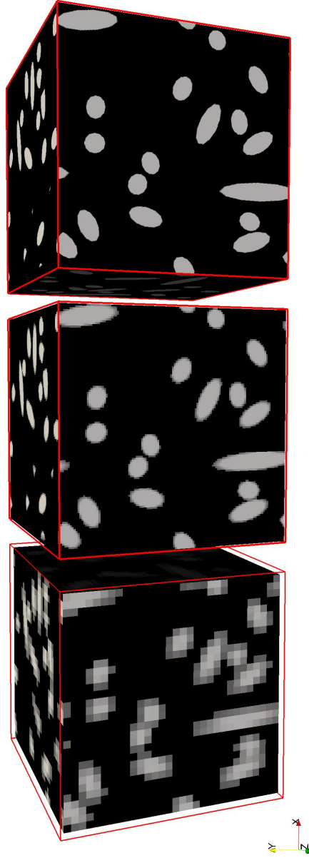
Figure 7: The same microstructure of length 133\mu\text{m} is discretized on grids of size N = 32 , N = 128 and N = 648 . Hence the corresponding total numbers of voxels are respectively 32^3 , 128^3 and 648^3 . Cross sections of cylindrical fibers are ellipses, except at edges.
