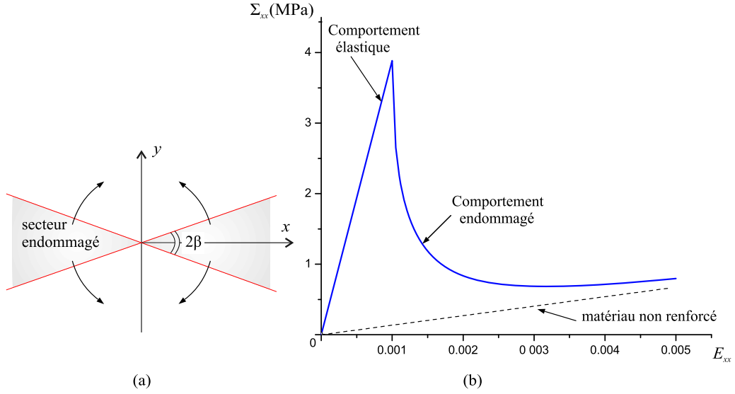
Fig. 5. (a) Evolution of the damaged zone. (b) Macroscopic behaviour (uniaxial macroscopic strain).
