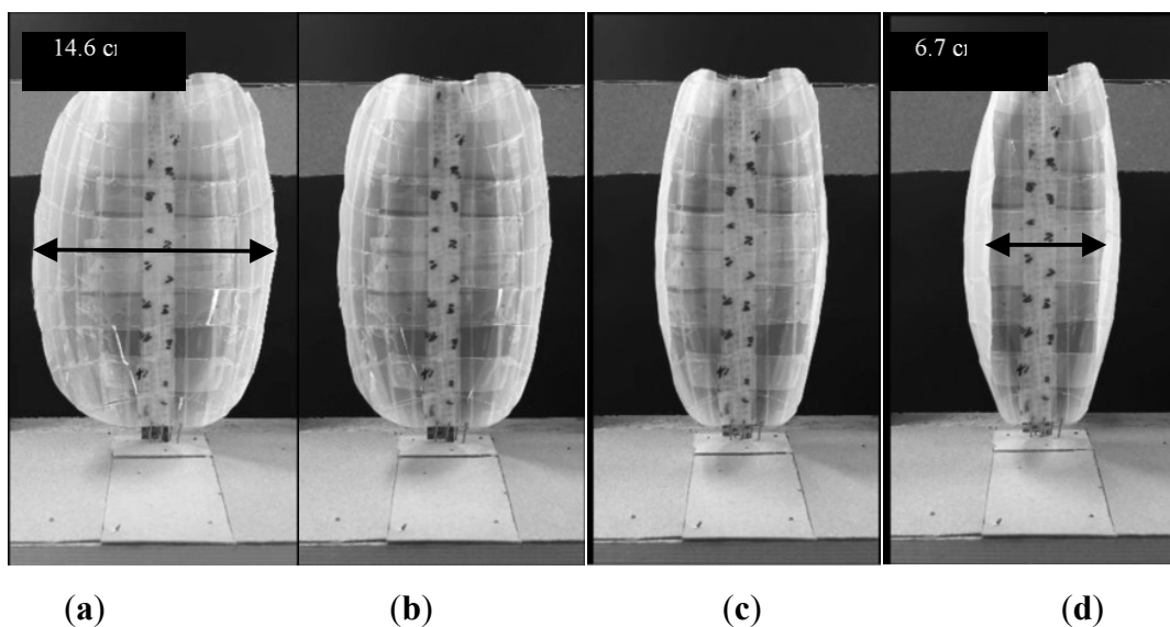
Figure 10. Physical small scale prototype, before (a) during (b), (c) and after (d) a temperature increase is applied to the connecting beam provides insight into the geometric and mechanical relationships between the beam and shell components.
