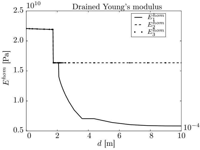
Figure 7: Evolution of the solid skeleton Young's modulus under uniaxial traction strain. R^1 = 1 \text{ mm} , f^1 = 0.1
