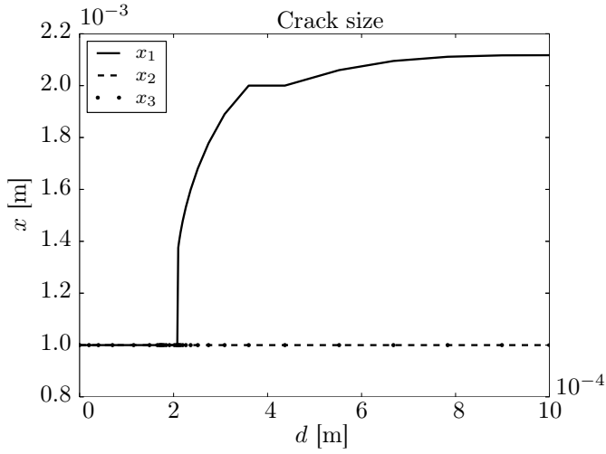
Figure 6: Evolution of the crack size under uniaxial traction strain. R^1 = 1 \text{ mm} , f^1 = 0.1
