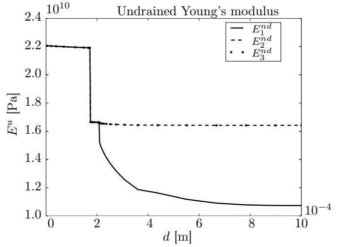
Figure 8: Evolution of the undrained Young's modulus under uniaxial traction strain. R^1 = 1 \text{ mm} , f^1 = 0.1
