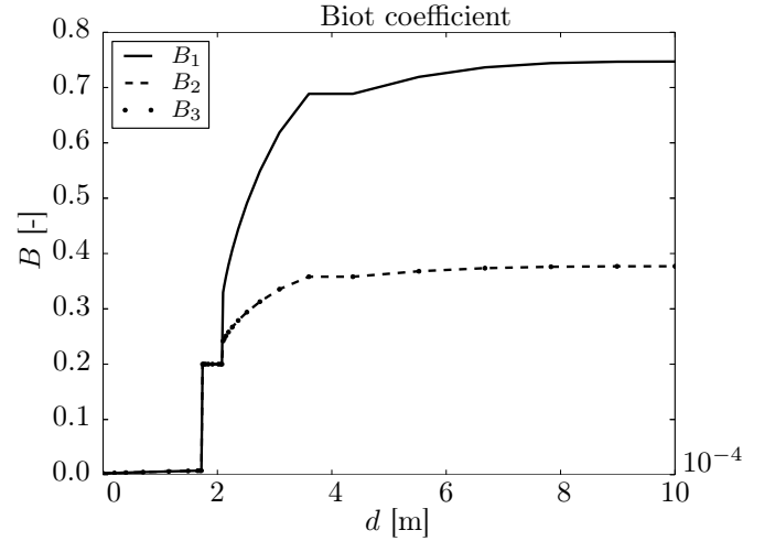
Figure 9: Evolution of Biot coefficients under uniaxial traction strain. R^1 = 1 \text{ mm} , f^1 = 0.1
