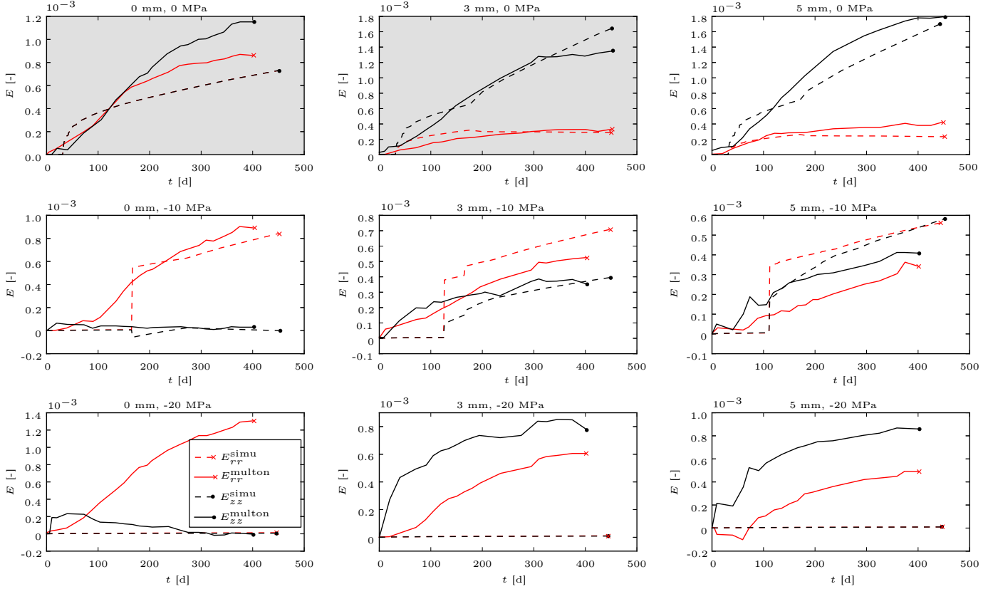
Figure 18: Identification of parameters on Multon's experiments. Strain. Grey plots: experiment used for the identification.
