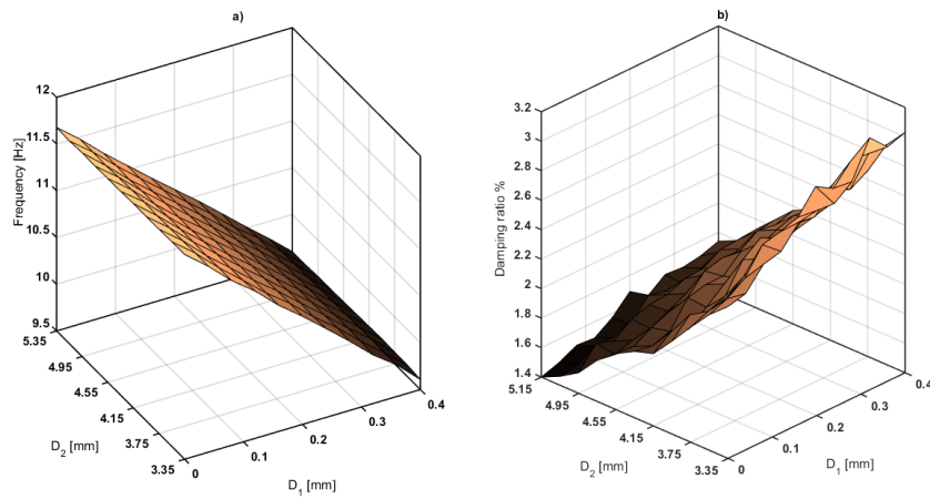
Figure 7 – a) TMD's damped frequency and b) damping ratio by varying cable stretching and magnet position
