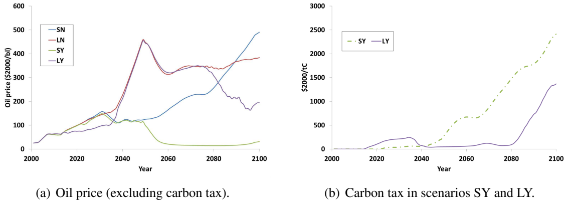
Figure 5: Oil price and carbon tax computed by Imacim-R model in the four scenarios. The carbon tax is applied everywhere around the world, and is computed so that \text{CO}_2 concentration is stabilized at 450 ppm in the long run (corresponding to a 550 ppm \text{CO}_2\text{eq.} stabilization). There is no carbon tax in Techno-economic scenarios SN and LN.
