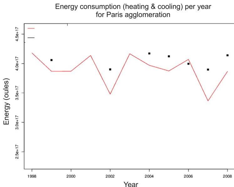
Fig. 7. Energy consumption for buildings (heating and cooling) in Paris urban area.
