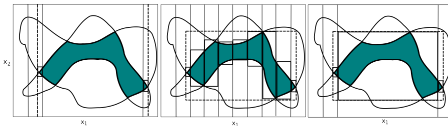
Fig. 1 Task of the var3B (left), varCID (center) and var3BCID (right) procedures applied to the interval [x_1] , with parameter s_{3b} set to 10 and s_{cid} set to 1. The darkened region corresponds to the solution set of the two constraints. The boxes in dotted lines are returned by the respective procedures.
