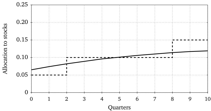
Figure 3: Path of optimal allocation to stocks for \alpha = 5 , X_0 = X_{(30)} , and T = 10 obtained by explicit solution (solid line) and by simulation and trial \{0.05, 0.10, 0.15, 0.20, 0.25\} grid (dashed line)
