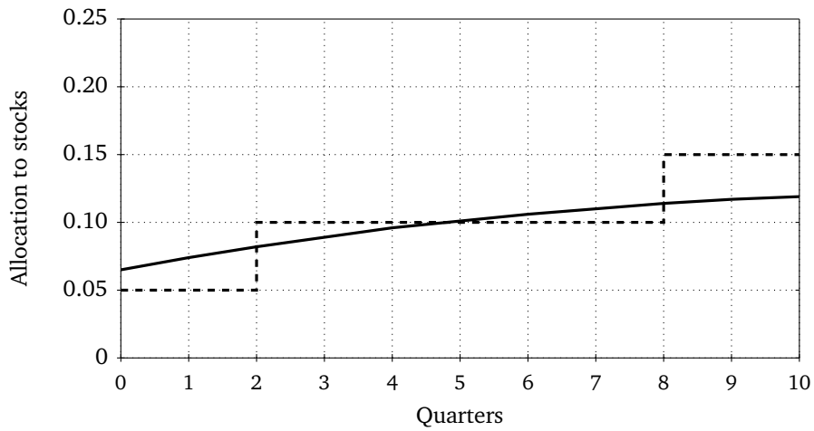
Figure 3: Path of optimal allocation to stocks for \sigma = 5 , X_0 = X_{(30)} , and T = 10 obtained by explicit solution (solid line) and by simulation and trial \{0.05, 0.10, 0.15, 0.20, 0.25\} grid (dashed line)
