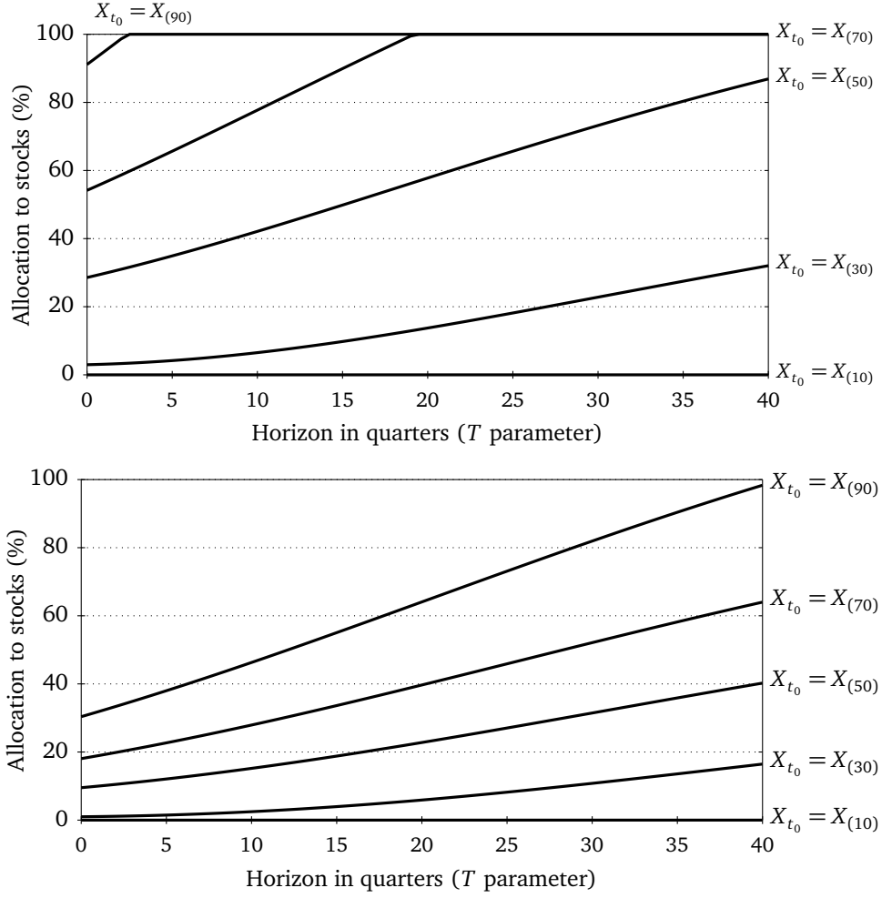
Figure 2: Optimal allocation to stocks as function of the horizon for \sigma = 5 (first panel) and for \sigma = 15 (second panel) for 5 different initial values of the Sharpe ratio X (as in table 2 or 3)
