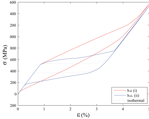
Figure 6: Stress-strain curves in NiTi for different thermal conditions
