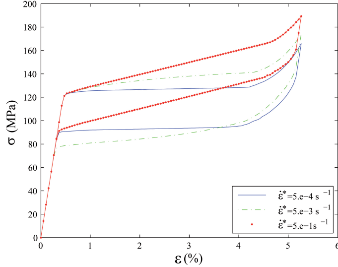
Figure 3: Stress-strain curves at several applied strain rates (CuAlNi).
