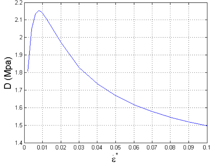
Figure 4: Size of the hysteresis loop as a function of the loading strain rate.
