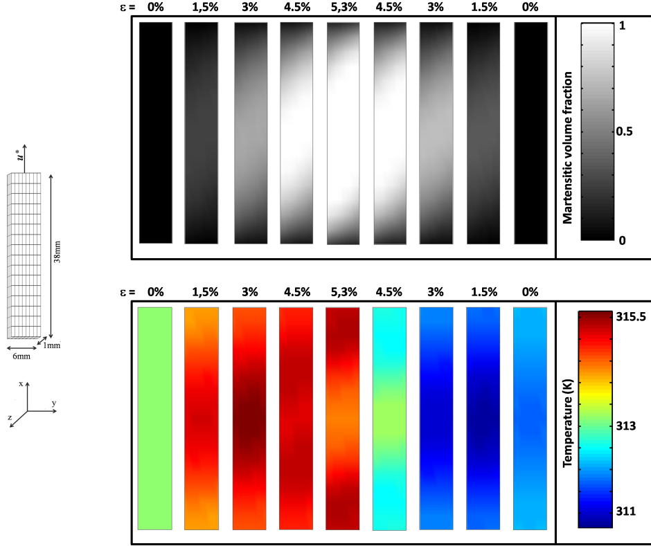
Figure 1: Phase transformation (top) and temperature distribution (bottom) in a CuAlNi rectangular sample loaded in traction.
