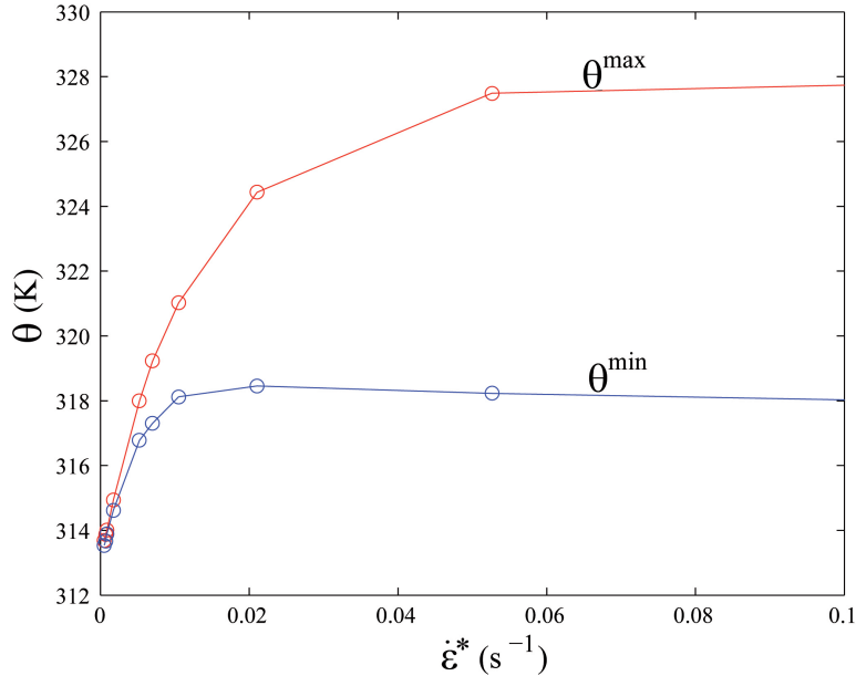
Figure 2: Maximum and minimum temperatures in the sample as a function of the loading strain rate.
