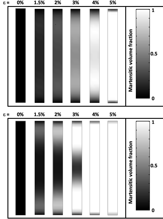
Figure 5: Phase transformation in NiTi, for two different thermal boundary conditions at the end sections: null heat flux (top) and prescribed temperature (bottom)
