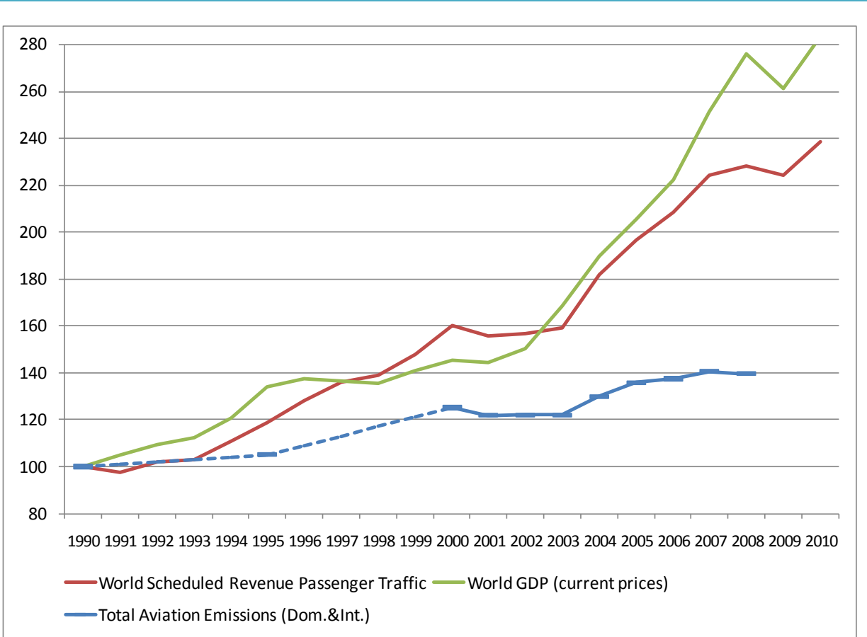
Figure 2 – CO 2 emissions from aviation, air transport demand and GDP per year, 1990-2010 (1990=100)
