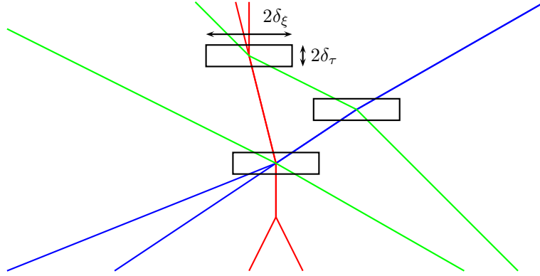
FIGURE 3. An example of set of (\delta_\xi, \delta_\tau) -boxes around the points of \mathcal{I}^{\text{coll}}(\mathbf{x}) .
