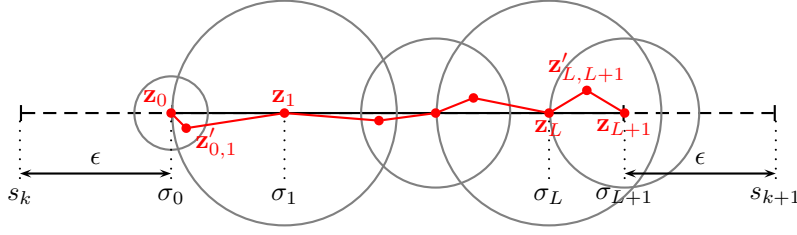
FIGURE 7. The segment S_k is drawn in dashed line, while the segment S_k^\epsilon is drawn in solid line. Gray circles stand for the open balls B_1(\mathbf{z}_l, \kappa(\mathbf{z}_l)) . The points \mathbf{z}'_{0,1}, \dots, \mathbf{z}'_{L,L+1} are chosen in the dense set \mathcal{G} in order to ensure that the difference between the length of the red path and the length (s_{k+1} - s_k - 2\epsilon)\|\mathbf{x} - \mathbf{y}\| of S_k^\epsilon be smaller than \eta .
