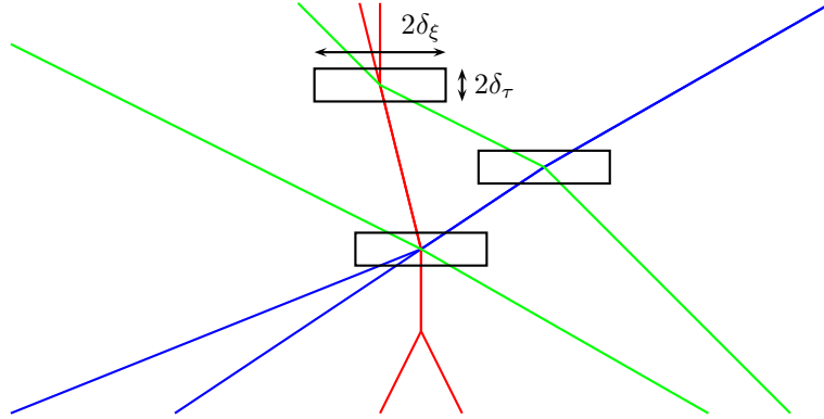
FIGURE 3. An example of set of (\delta_\xi, \delta_\tau) -boxes around the points of I^{\text{coll}}(\mathbf{x}) .
