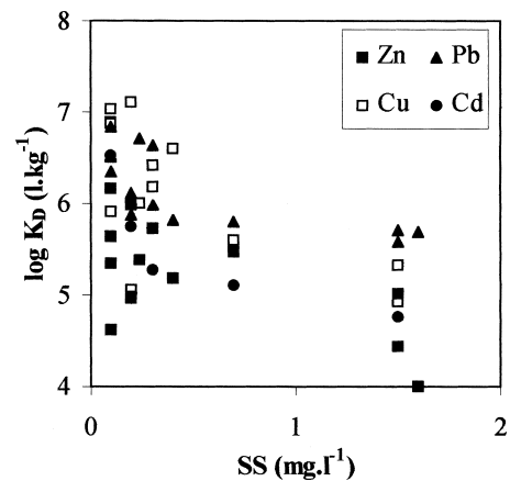
Fig. 3. Correlation between the logarithm of metal distribution factor K_D (l kg -1 ) and the SS level (mg l -1 ) in rain samples at Paris centre.
