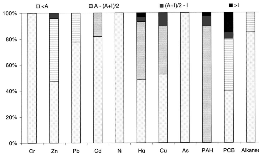
Fig. 2. Statistical distribution of the number of sediment samples presenting a contamination in heavy metals or organic micropollutants below ( <A ) the Alert value of the Dutch decree on the quality of sediments, above ( >I ) the Intervention value of this decree, or within these two values.
