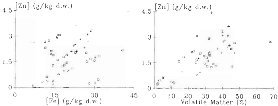
Fig. 2. Correlations between total particulate zinc and either total particulate iron, or volatile matter Sites: ○ : 1, × : 2, * : 3, △ : 4, + : 5, □ : 6, ◻ : 7, X : 8 (see text for sample identification)
