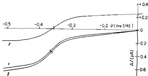
Fig. 7. Differential d.c. voltammograms of benzyl-viologen on R.P.D.E. in glycine buffer (pH 9.5). (1) 40 \mu\text{M} benzyl-viologen, (2) as (1) with 0.5 mM NADH and (3) as (2) with 1 \mu\text{M} xanthine oxidase. Background base current was subtracted.
