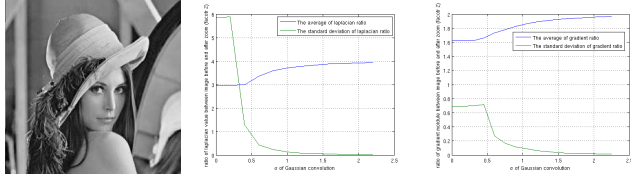
Fig. 2: Image on the left is convolved by a Gaussian function with standard deviation \sigma before it is up-sampled by factor 2. The Laplacian value and gradient modulus before and after the up-sampling are compared. Middle: the average and standard deviation of ratio of the Laplacian value before and after 2-up-sampling. Right: the average and standard deviation of ratio of gradient modulus before and after 2-up-sampling.
