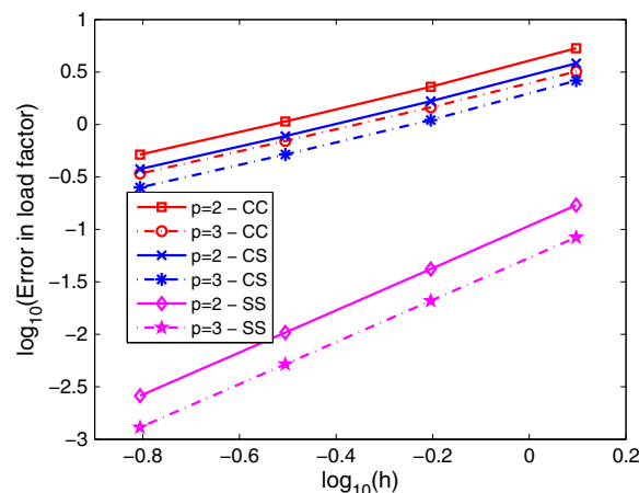
Figure 7 Convergence rate of limit load factors of beams.
