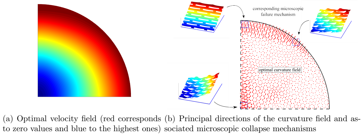
Figure 6: Optimal kinematic fields for the slotted circular plate problem
