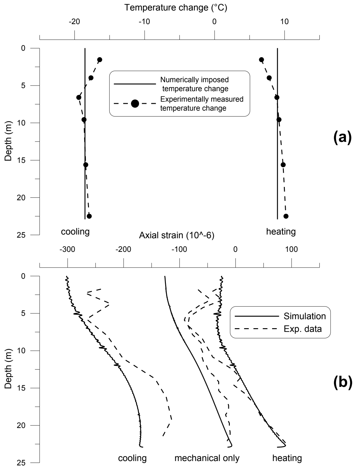
Figure 5. Test presented by Bourne-Webb et al. (2009): (a) Profile of temperature along the pile; (b) Pile axial strain distribution.
